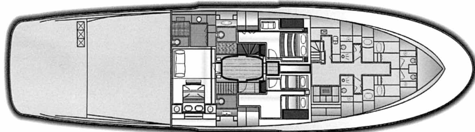
LOWER DECK
